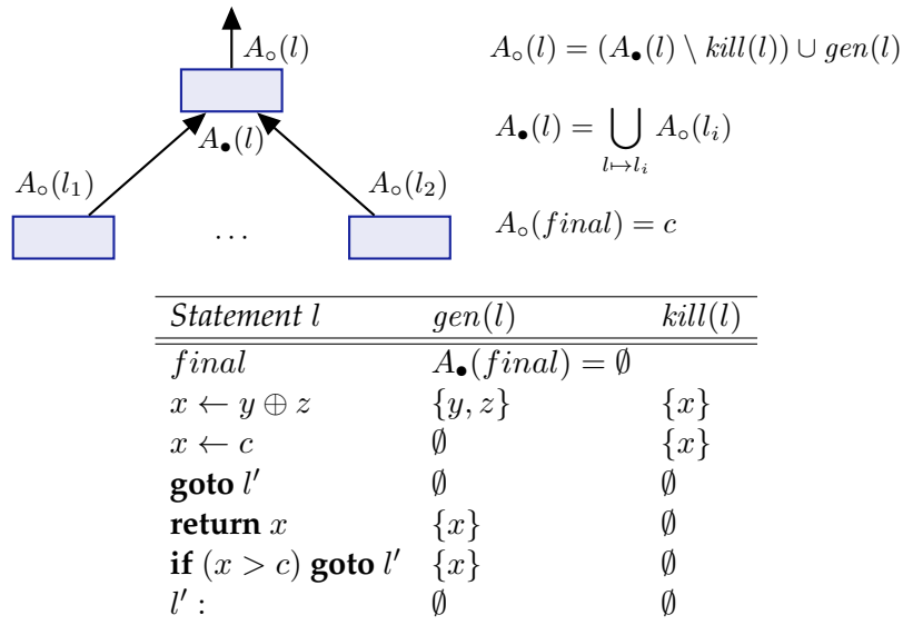
Figure 2: Dataflow analysis for live-in A_o(l) and live-out A_{\bullet}(l) variables
