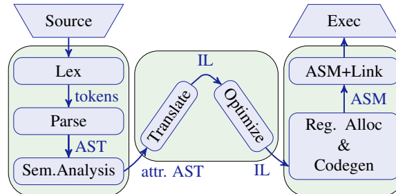
Figure 1: Structure of a compiler
